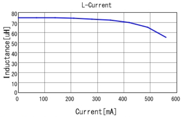
#A921CY-820M=P3 L-Current 20degC
