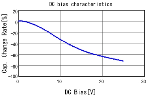
GRM188R61E105KAAD C-DC bias capchange, 25.0degC, A
