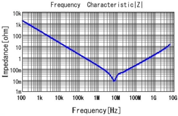
GRM188R61E105KAAD |Z| DCOV, 25degC
