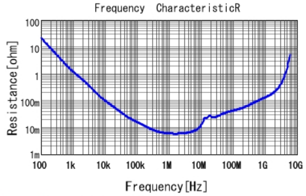
GRM188R61E105KAAD R DCOV, 25degC
