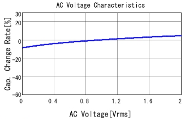
GRM188R61E105KAAD C-AC Voltage capchange, DCOV, 25
