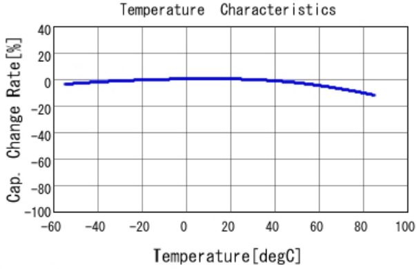
GRM188R61E105KAAD C-Temp. capchange, DC0.0V, AC1.C
