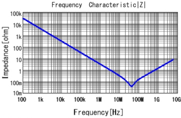
■ GRM033R60J683KE19 |Z| DCOV, 25degC
