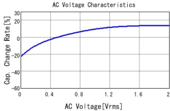
■ GRM033R60J683KE19 C-AC Voltage capchange, DCOV, 25.0d
