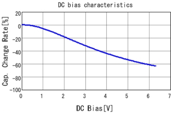
■ GRM033R60J683KE19 C-DC bias capchange, 25.0degC, AC0.
