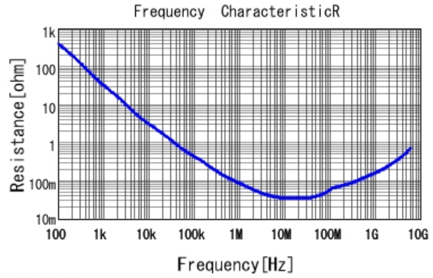
■ GRM033R60J683KE19 R DCOV, 25degC
