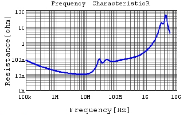
GRM55DR72J224KW01 R DCOV, 25degC
