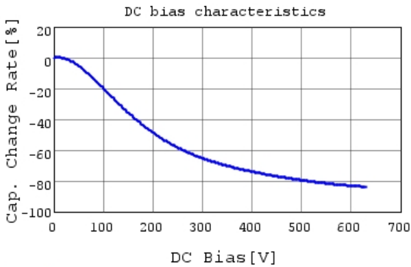
GRM55DR72J224KW01 C-DC bias capchange, 25.0c
