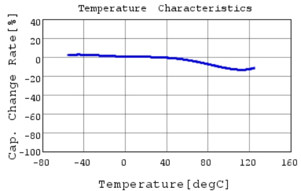
GRM55DR72J224KW01 C-Temp. capchange, DCOV, 1
