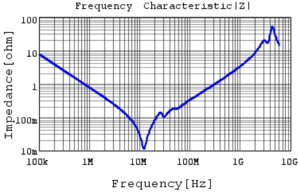
GRM55DR72J224KW01 |Z| DCOV, 25degC
