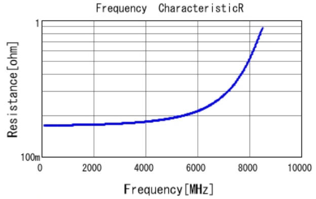
GQM1875C2E2R2BB12 R DCOV, 25degC
