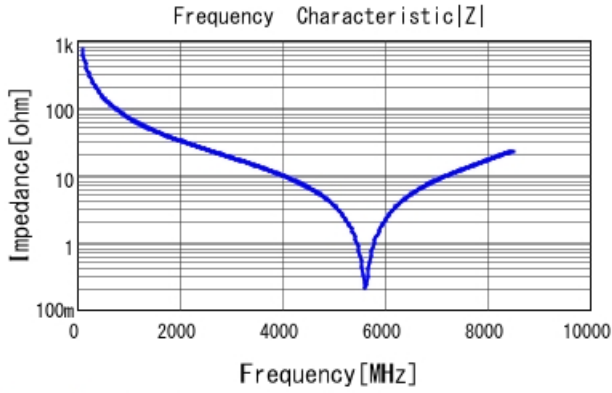
GQM1875C2E2R2BB12 |Z| DCOV, 25degC
