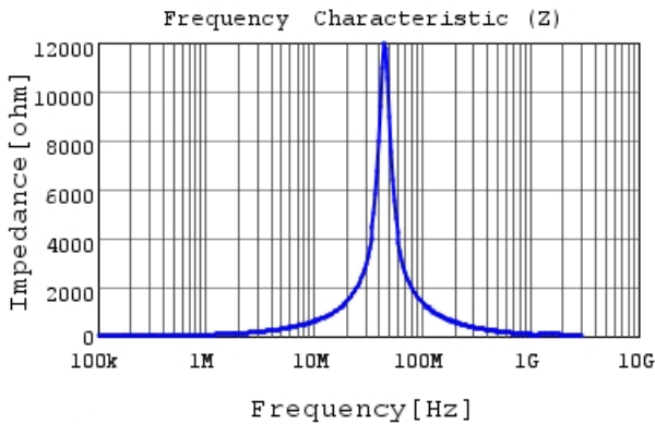
LQH2HPZ100MGR |Z|
