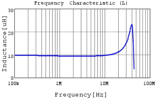
LQH2HPZ100MGR L
