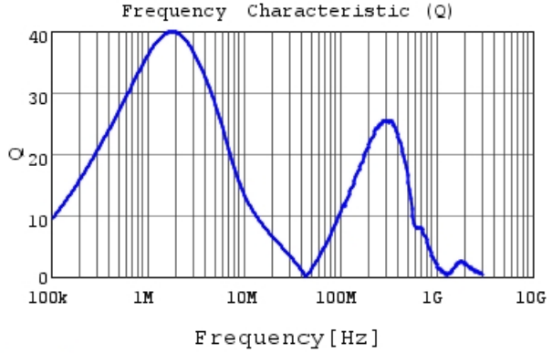
LQH2HPZ100MGR Q
