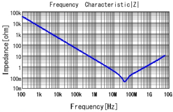
GRM155R61A473KA01 |Z| DCOV, 25degC
