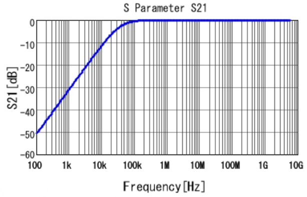
GRM155R61A473KA01 S21 DC0V, 25degC
