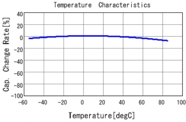
GRM155R61A473KA01 C-Temp. capchange, DC0.0V, AC1.C
