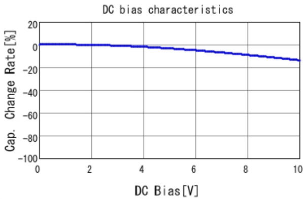
GRM155R61A473KA01 C-DC bias capchange, 25.0degC, A
