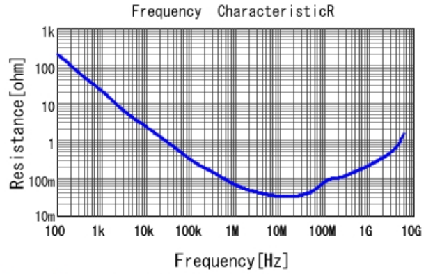
GRM155R61A473KA01 R DCOV, 25degC
