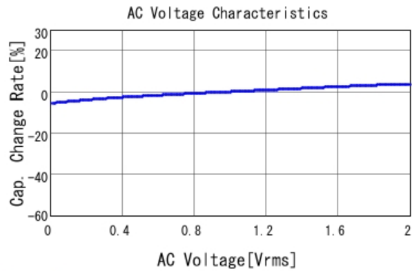
GRM155R61A473KA01 C-AC Voltage capchange, DCOV, 25
