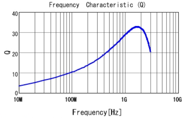
LQG15HH9N1G02 Q
