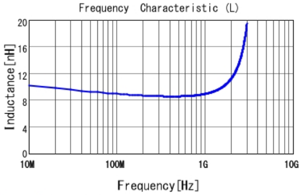
LQG15HH9N1G02 L
