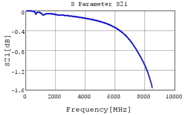
GCM1885C2A391JA16 S21 DCOV, 25degC
