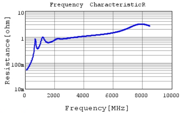
GCM1885C2A391JA16 R DC0V, 25degC
