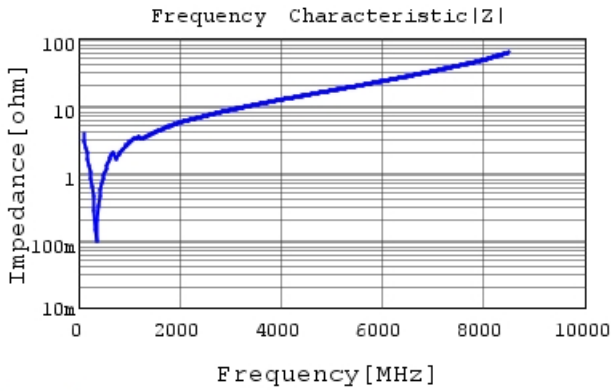
GCM1885C2A391JA16 |Z| DC0V, 25degC
