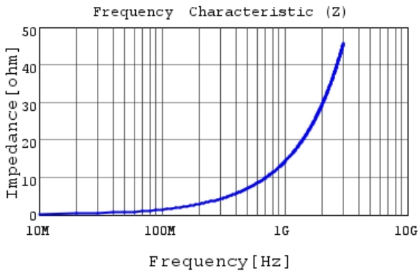
LQG15WH2N3S02 |Z|
