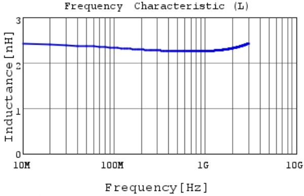
LQG15WH2N3S02 L
