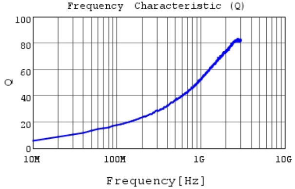
LQG15WH2N8C02 Q
