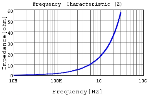
LQG15WH2N8C02 |Z|
