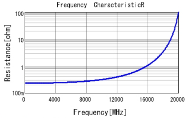
GJM1555C1H1R0BB01 R DCOV, 25degC
