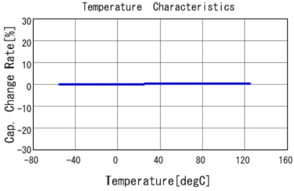
GJM1555C1H1R0BB01 C-Temp. capchange, DCOV, AC1Vrms
