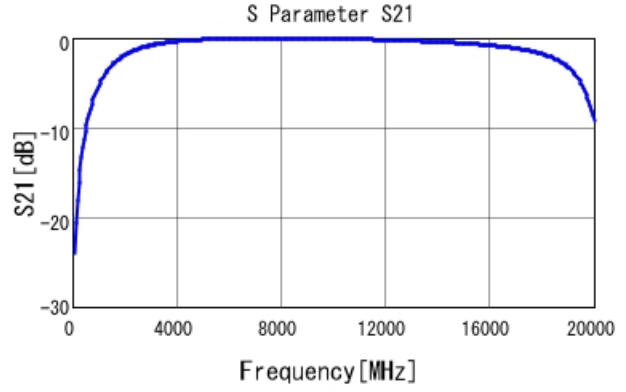
GJM1555C1H1R0BB01 S21 DCOV, 25degC
