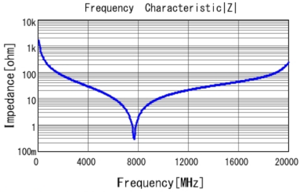
GJM1555C1H1R0BB01 |Z| DCOV, 25degC
