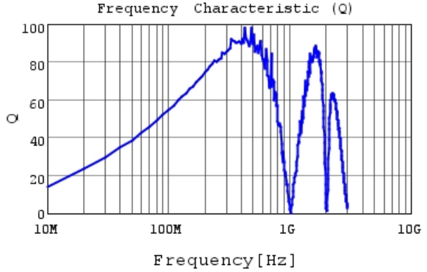
LQW2UASR15J0C Q
