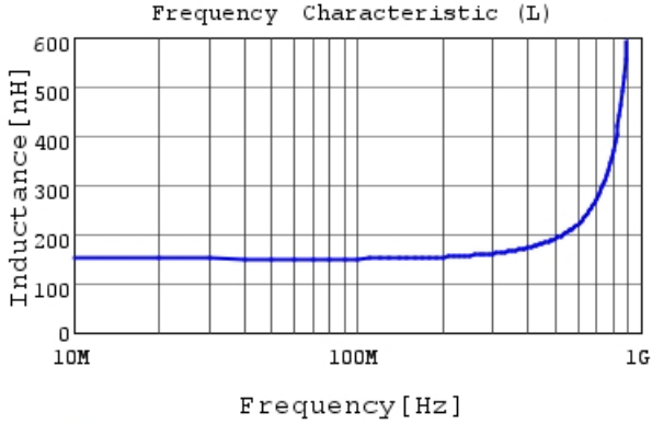
LQW2UASR15J0C L
