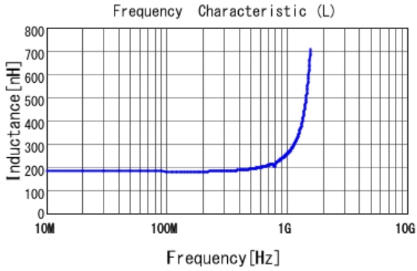
LQW15AWR18H80 L
