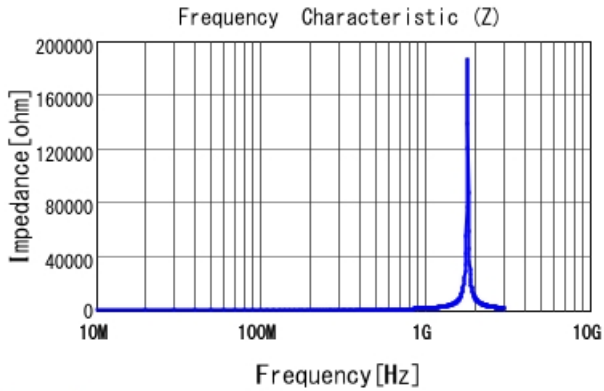
LQW15AWR18H80 |Z|
