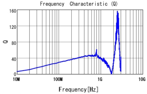
LQW15AWR18H80 Q
