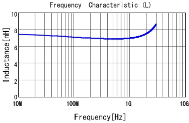
LQP03HQ6N8J02 L
