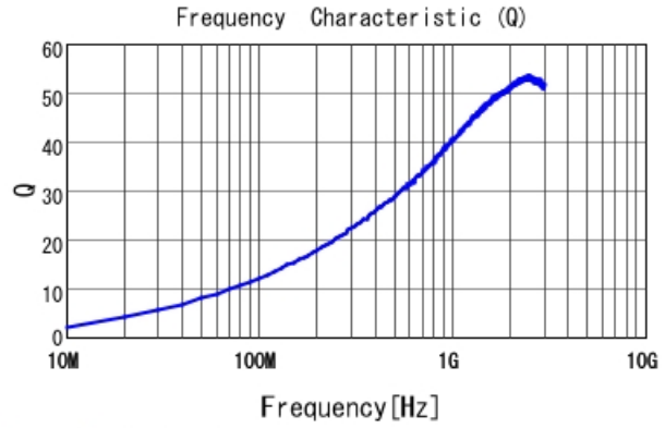
LQP03HQ6N8J02 Q
