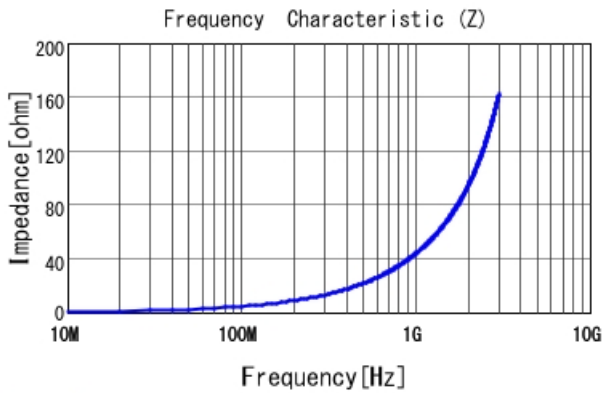
LQP03HQ6N8J02 |Z|
