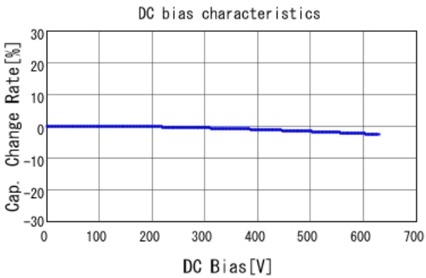
■ GRM31A7U2J561JW31 C-DC bias capchange, 25.0degC, AC1V
