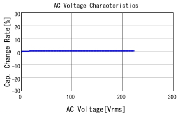
■ GRM31A7U2J561JW31 C-AC Voltage capchange, DCOV, 25.0d
