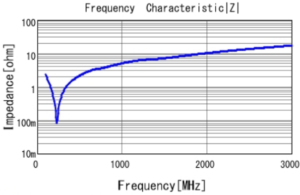
■ GRM31A7U2J561JW31 |Z| DCOV, 25degC
