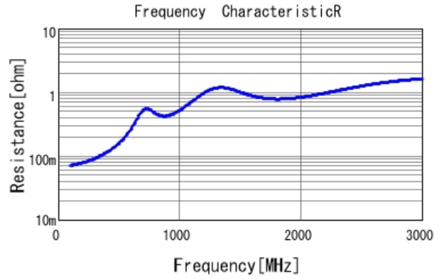
■ GRM31A7U2J561JW31 R DCOV, 25degC
