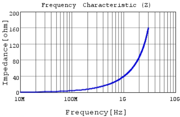
LQG15WH6N2C02 |Z|
