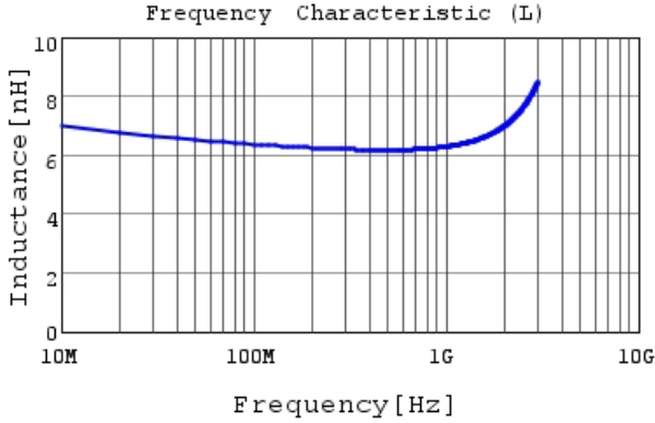
LQG15WH6N2C02 L
