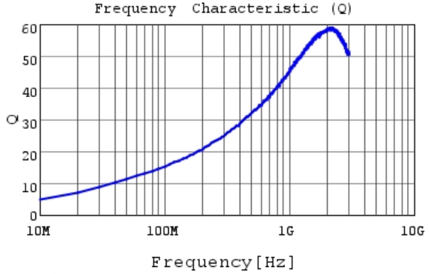
LQG15WH6N2C02 Q
