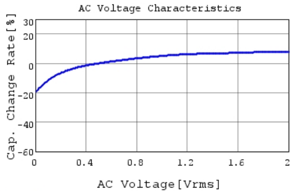
GRM155C70J225KE11 C-AC Voltage capchange, DC
