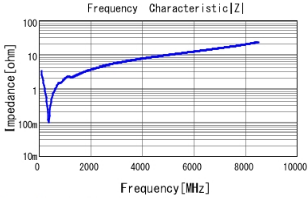
GRM1555C1H471GA01 |Z| DCOV, 25degC
