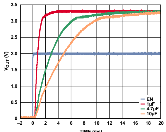
Figure 40. V_{OUT} Start-Up Time Behavior at Various Values of C_{BYF} , V_{OUT} = 3.3 \text{ V}
