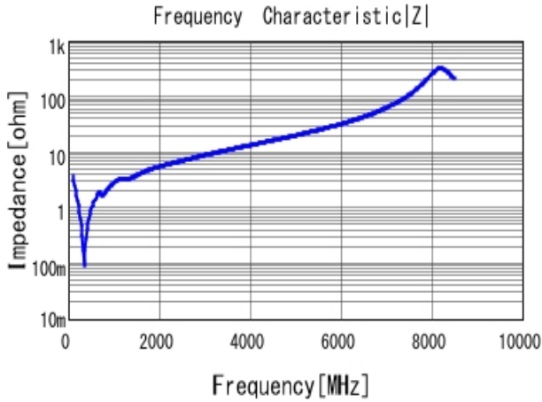
■ GRM1885C1H391JA01 |Z| DCOV, 25degC
