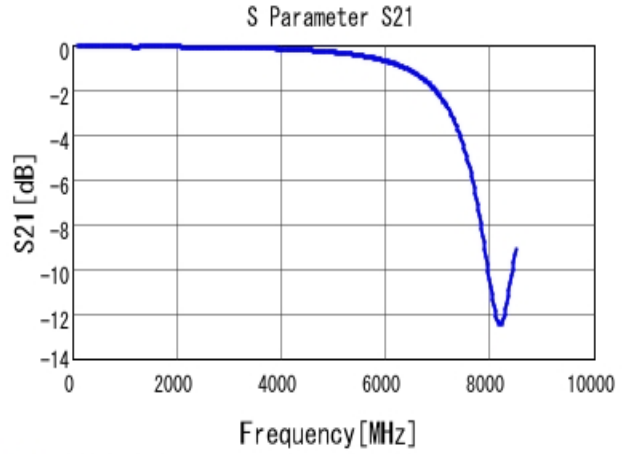
■ GRM1885C1H391JA01 S21 DCOV, 25degC
