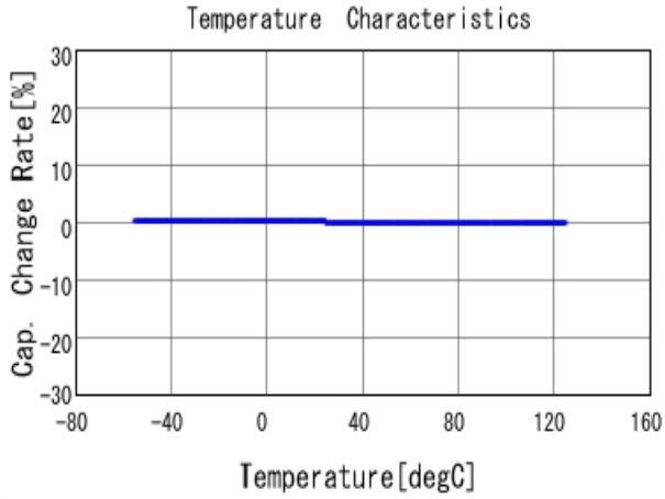
■ GRM1885C1H391JA01 C-Temp. capchange, DCOV, AC1Vrms
