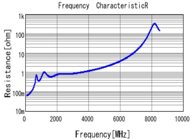
■ GRM1885C1H391JA01 R DCOV, 25degC
