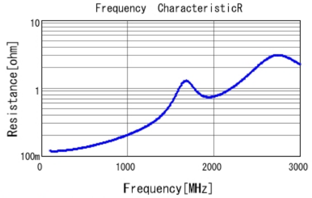
GCM21A5C2E101JX01 R DCOV, 25degC
