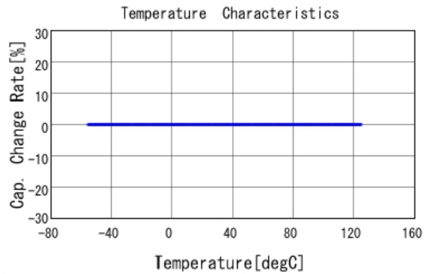
GCM21A5C2E101JX01 C-Temp. capchange, DCOV, AC1Vrms
