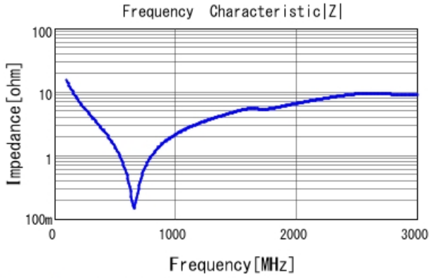
GCM21A5C2E101JX01 |Z| DCOV, 25degC
