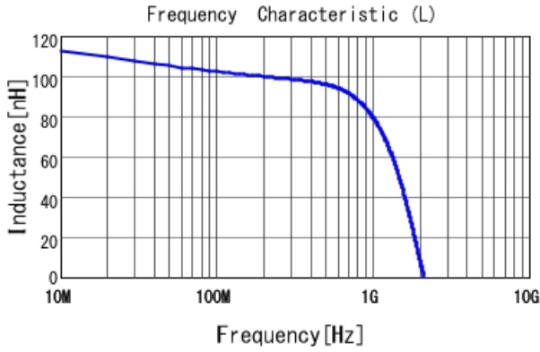
LQW15CAR11J00 L
