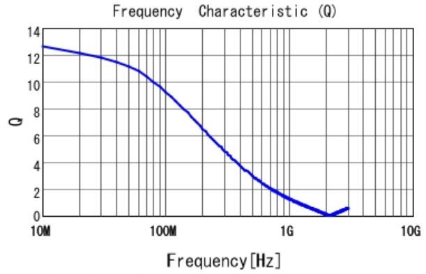
LQW15CAR11J00 Q
