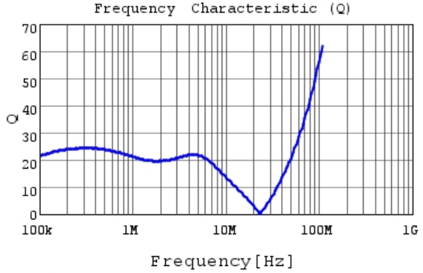
LQH5BPPB220MT0 Q
