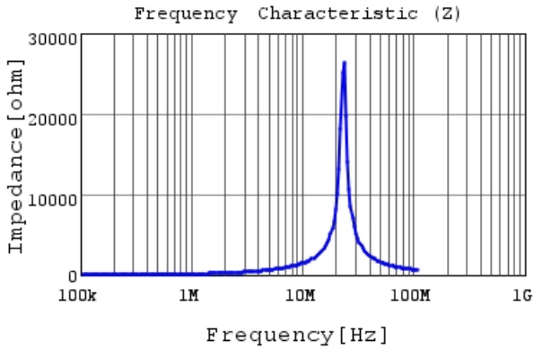
LQH5BPPB220MT0 |Z|
