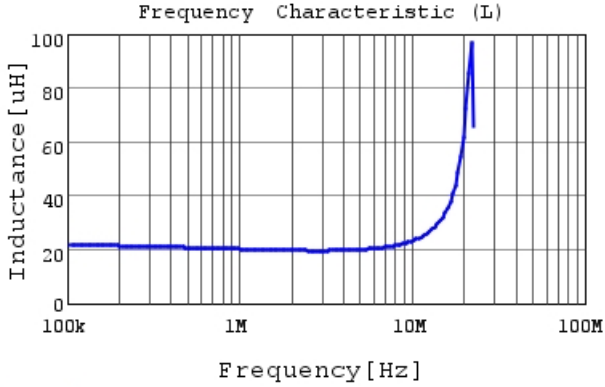
LQH5BPPB220MT0 L
