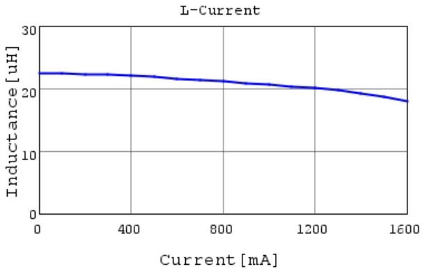
LQH5BPPB220MT0 L-Current 20degC
