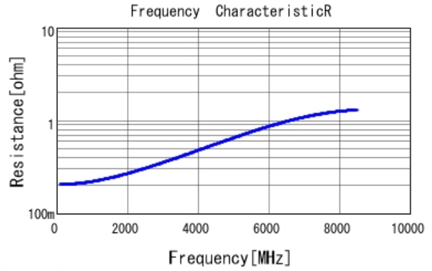
GRM0335C1E5R6CA01 R DCOV, 25degC
