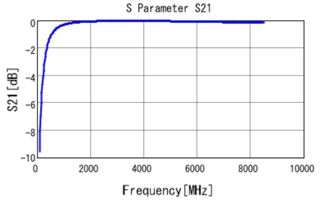
GRM0335C1E5R6CA01 S21 DCOV, 25degC
