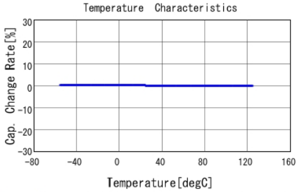
GRM0335C1E5R6CA01 C-Temp. capchange, DCOV, AC1Vrms
