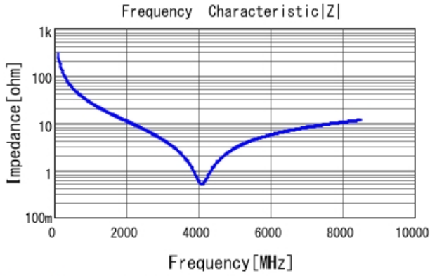
GRM0335C1E5R6CA01 |Z| DCOV, 25degC
