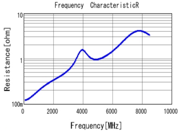
■ GRM1555C1H220JA01 R DCOV, 25degC
