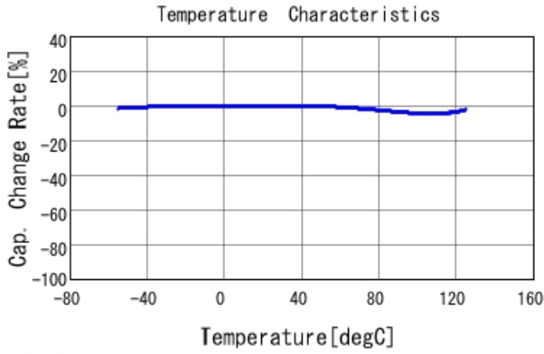
■ GRM033R71H101MA12 C-Temp. capchange, DCO. 0V, AC1. 0Vrm
