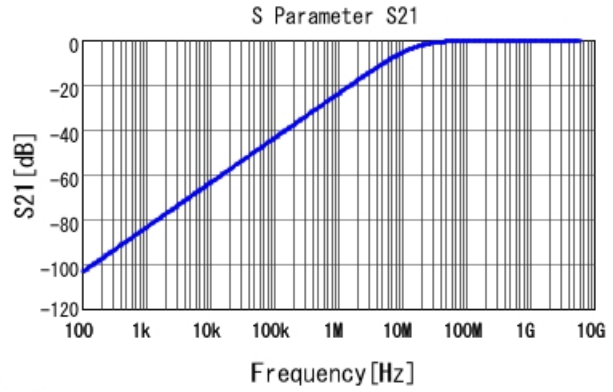
■ GRM033R71H101MA12 S21 DCOV, 25degC
