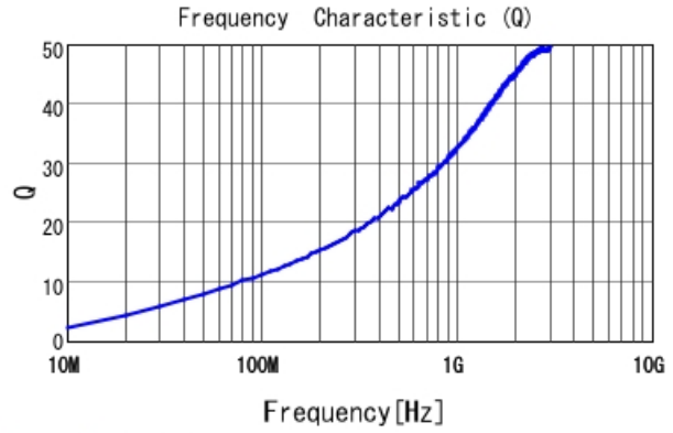
LQP03TN3N0CZ2 Q
