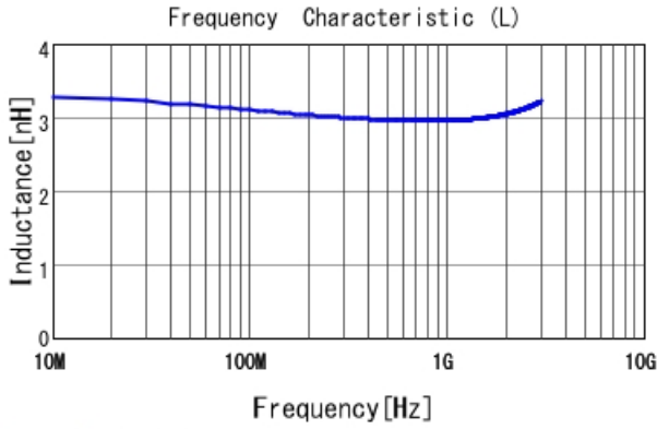
LQP03TN3N0CZ2 L
