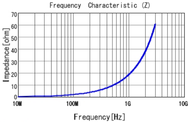
LQP03TN3N0CZ2 |Z|
