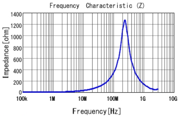
LQH32PZR47NN0 |Z|
