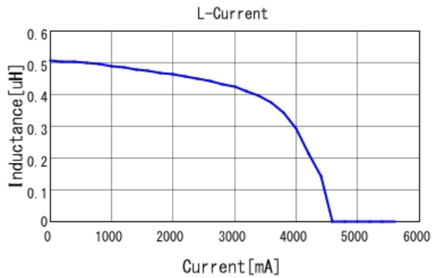
LQH32PZR47NN0 L-Current 20degC
