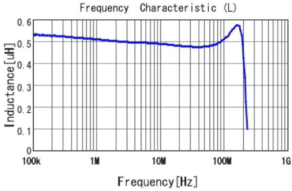
LQH32PZR47NN0 L
