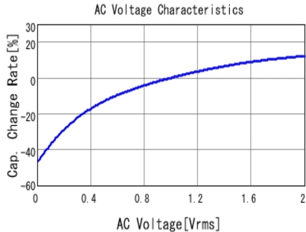
■ GRM155R61C474KE01 C-AC Voltage capchange, DCOV, 25.0d
