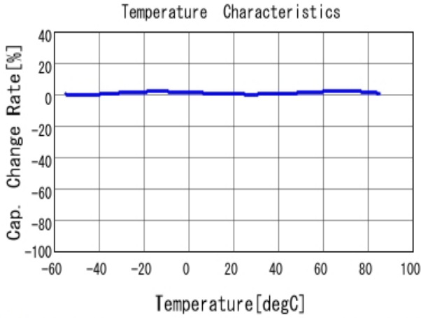
■ GRM155R61C474KE01 C-Temp. capchange, DC0.0V, AC1.0V r m
