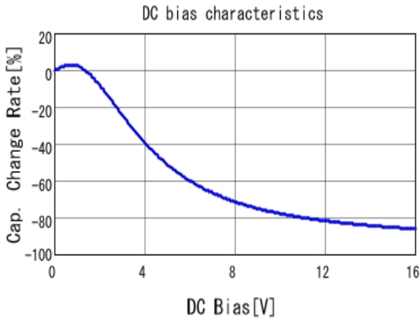
■ GRM155R61C474KE01 C-DC bias capchange, 25.0degC, AC1.
