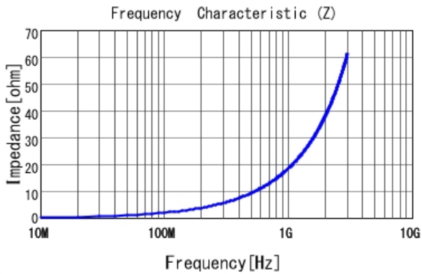
LQG15HN3N0B02 |Z|
