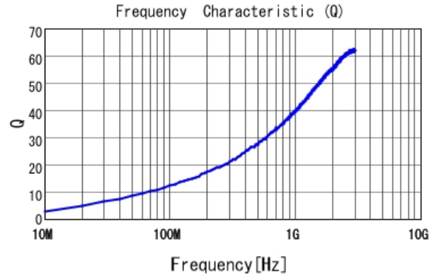
LQG15HN3N0B02 Q
