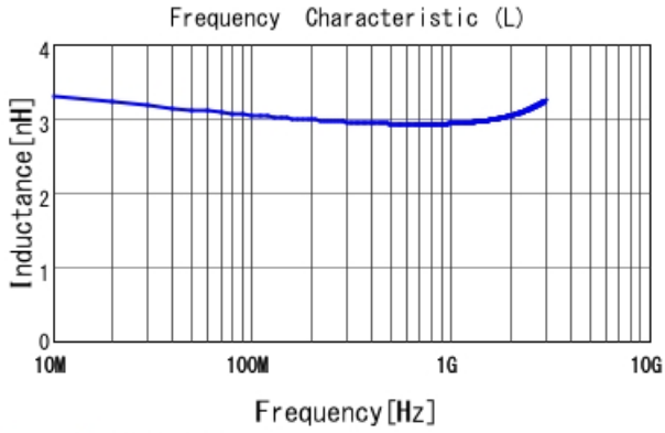
LQG15HN3N0B02 L
