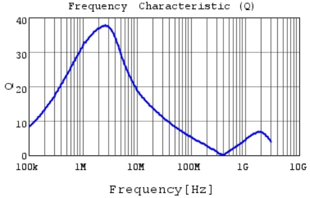
LQH32NH1R0M23 Q
