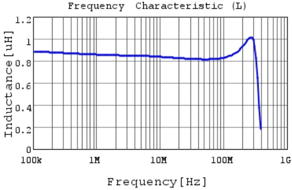
LQH32NH1R0M23 L
