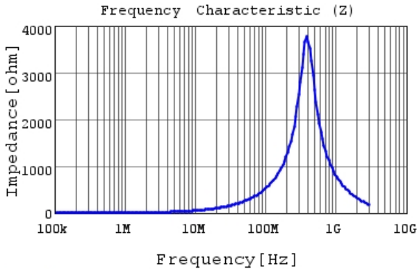
LQH32NH1R0M23 |Z|
