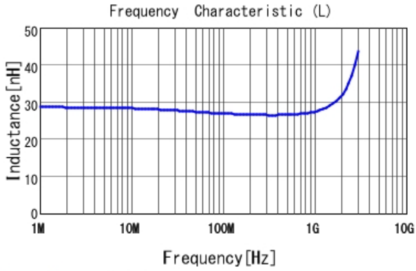
LQW15AN27NJ8Z L
