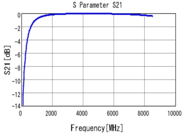
■ GRM1555C1H3R3CA01 S21 DCOV, 25degC
