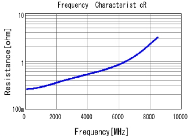
■ GRM1555C1H3R3CA01 R DC0V, 25degC
