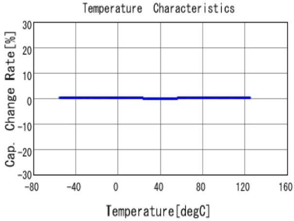
■ GRM1555C1H3R3CA01 C-Temp. capchange, DCOV, AC1Vrms
