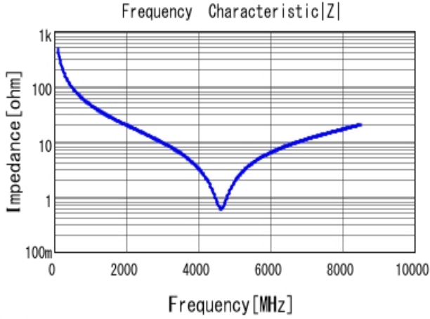
■ GRM1555C1H3R3CA01 |Z| DC0V, 25degC
