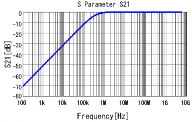
■ GRM033R61E472MA12 S21 DCOV, 25degC
