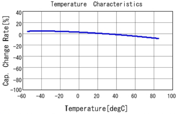
■ GRM033R61E472MA12 C-Temp. capchange, DCO. 0V, AC1. 0Vrm
