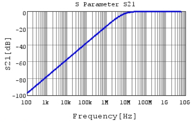
GRM155R72A221KA01 S21 DC0V, 25degC
