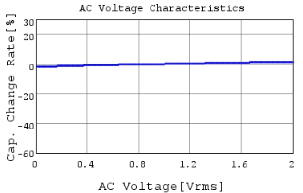
GRM155R72A221KA01 C-AC Voltage capchange, Dc
