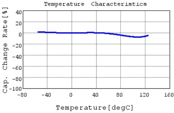
GRM155R72A221KA01 C-Temp. capchange, DC0.0V,
