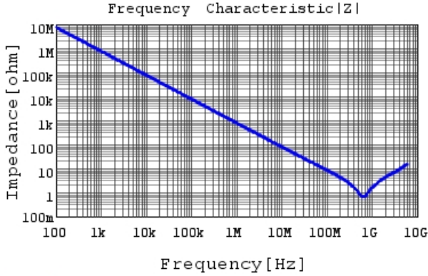
GRM155R72A221KA01 |Z| DCOV, 25degC
