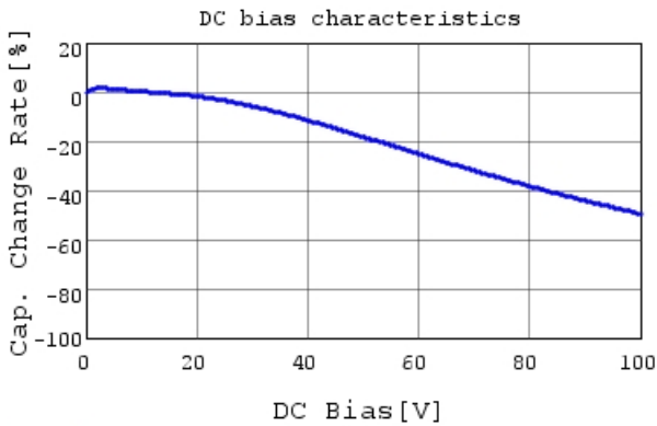
GRM155R72A221KA01 C-DC bias capchange, 25.0c
