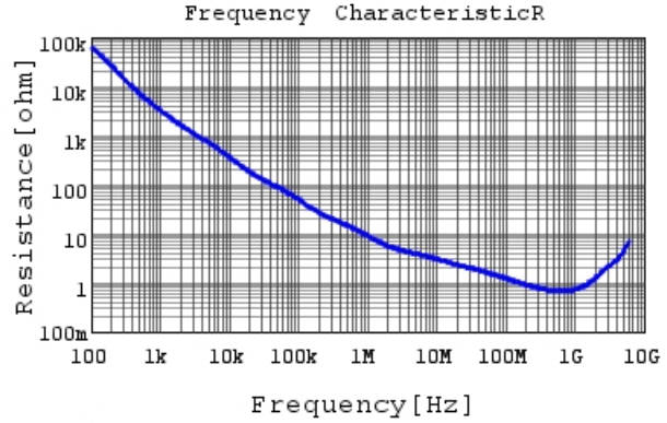
GRM155R72A221KA01 R DCOV, 25degC
