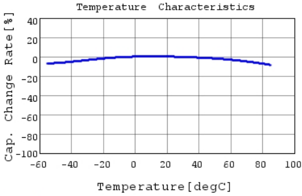
GRM033R61E104KE14 C-Temp. capchange, DC0.0V,
