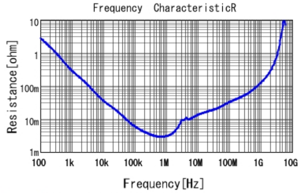
GRT21BR60J226ME13 R DCOV, 25degC
