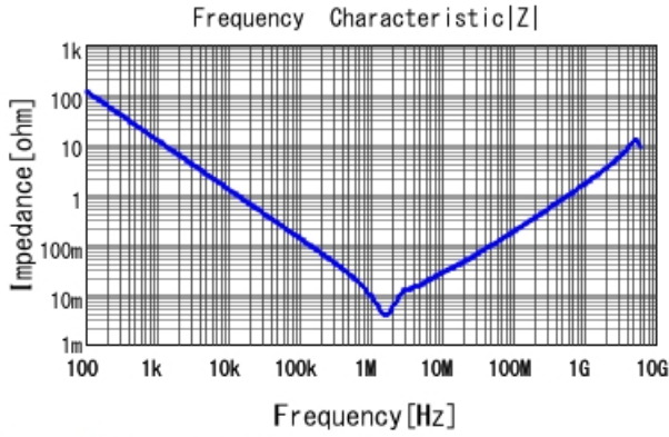
GRT21BR60J226ME13 |Z| DCOV, 25degC
