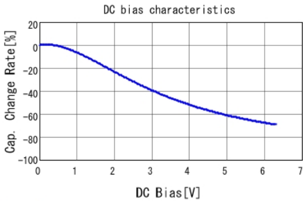
GRT21BR60J226ME13 C-DC bias capchange, 25.0degC, A
