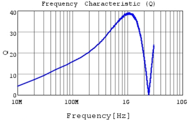
LQG15WH33NJ02 Q
