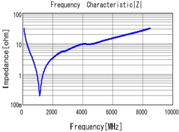
■ GRM1555C1H510JA01 |Z| DCOV, 25degC
