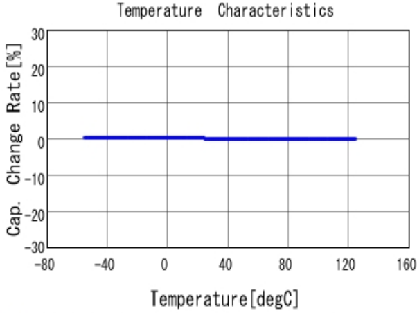
■ GRM1555C1H510JA01 C-Temp. capchange, DCOV, AC1Vrms
