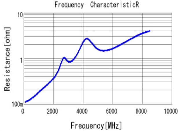
■ GRM1555C1H510JA01 R DCOV, 25degC
