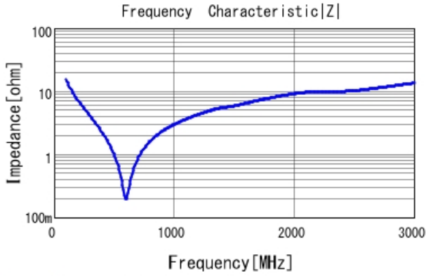
GRM21A7U2E101JW31 |Z| DCOV, 25degC
