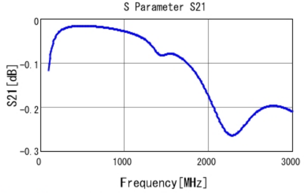
GRM21A7U2E101JW31 S21 DCOV, 25degC
