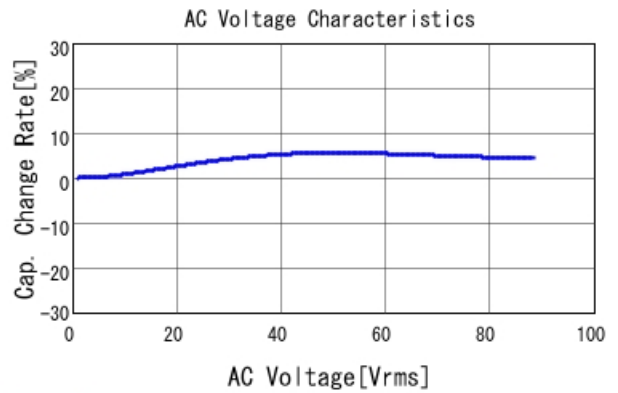
GRM21A7U2E101JW31 C-AC Voltage capchange, DCOV, 25
