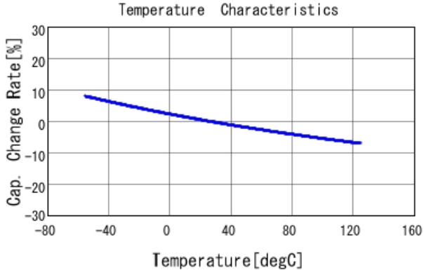
GRM21A7U2E101JW31 C-Temp. capchange, DCOV, AC1Vrms
