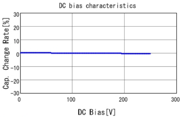
GRM21A7U2E101JW31 C-DC bias capchange, 25.0degC, A
