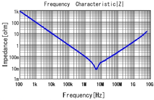
GRM188R61A225KE34 |Z| DCOV, 25degC
