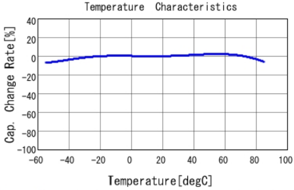
GRM188R61A225KE34 C-Temp. capchange, DC0.0V, AC0.5
