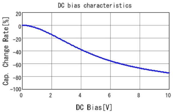
GRM188R61A225KE34 C-DC bias capchange, 25.0degC, A
