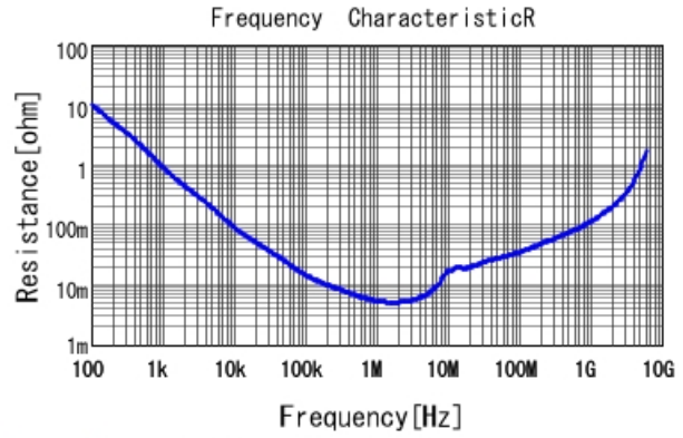
GRM188R61A225KE34 R DCOV, 25degC
