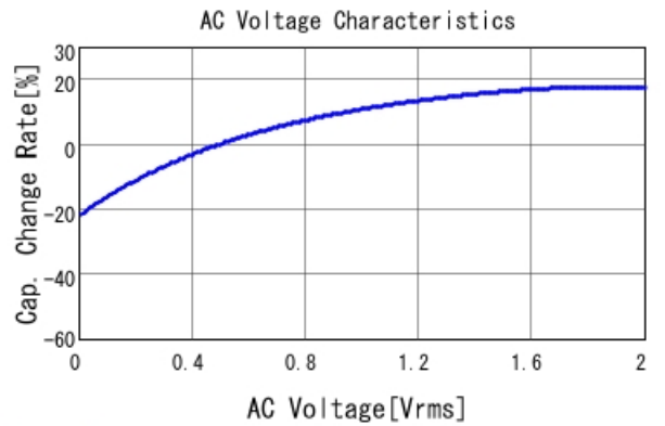
GRM188R61A225KE34 C-AC Voltage capchange, DCOV, 25
