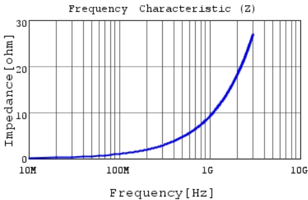
LQP02HQ1N5W02 |Z|
