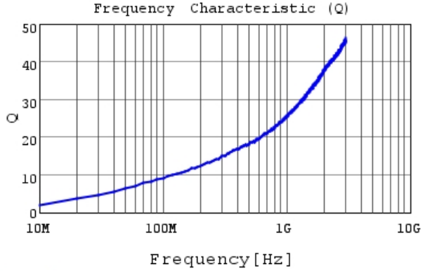
LQP02HQ1N5W02 Q
