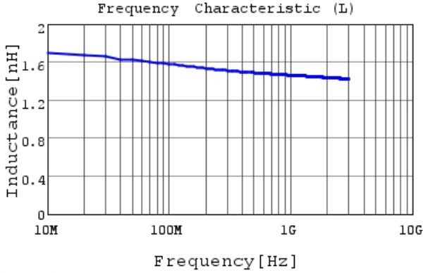
LQP02HQ1N5W02 L
