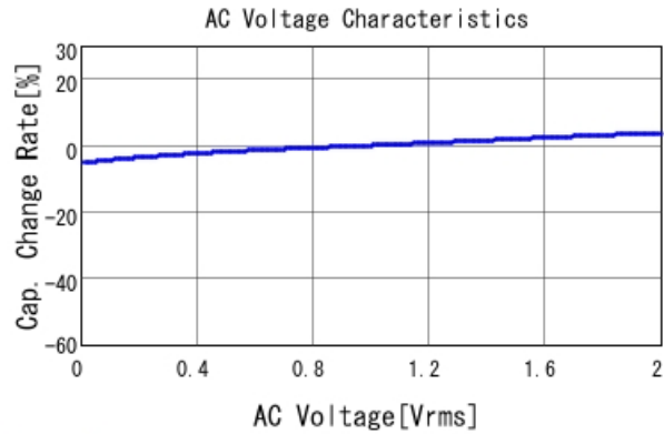
GRM319R71A105KA01 C-AC Voltage capchange, DCOV, 25
