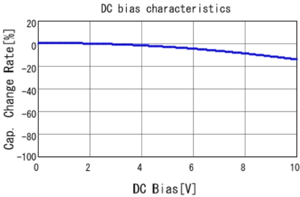
GRM319R71A105KA01 C-DC bias capchange, 25.0degC, A
