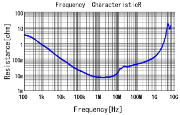
GRM319R71A105KA01 R DCOV, 25degC
