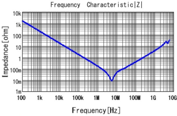
GRM319R71A105KA01 |Z| DCOV, 25degC
