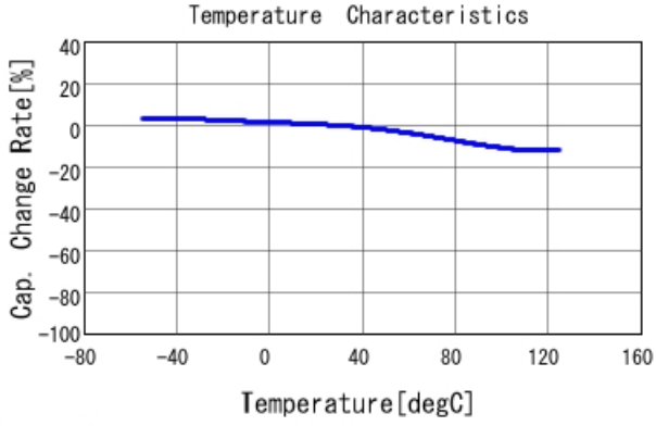
GRM319R71A105KA01 C-Temp. capchange, DC0.0V, AC1.C
