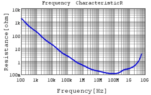
GCM155L81H472KA37 R DC0V, 25degC
