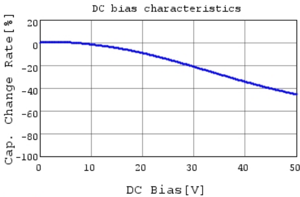
GCM155L81H472KA37 C-DC bias capchange, 25.0c
