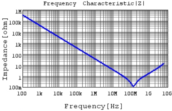
GCM155L81H472KA37 |Z| DC0V, 25degC
