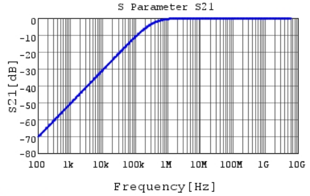
GCM155L81H472KA37 S21 DC0V, 25degC
