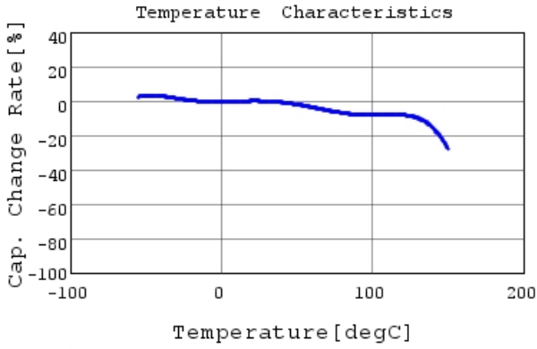
GCM155L81H472KA37 C-Temp. capchange, DC0.0V,
