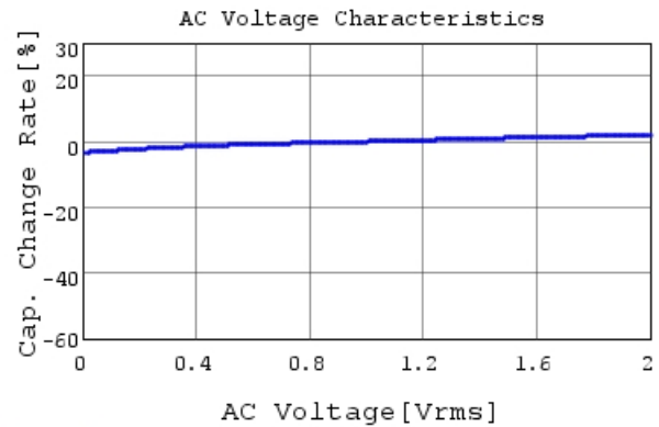
GCM155L81H472KA37 C-AC Voltage capchange, DC
