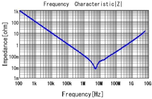
■ GRM188C71C225KE11 |Z| DCOV, 25degC
