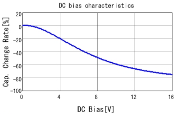
■ GRM188C71C225KE11 C-DC bias capchange, 25.0degC, AC1V
