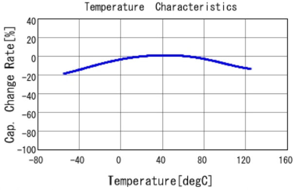
■ GRM188C71C225KE11 C-Temp. capchange, DCO. 0V, ACO. 2Vrm
