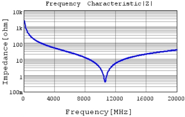
GJM0335C1ER70BB01 |Z| DC0V, 25degC
