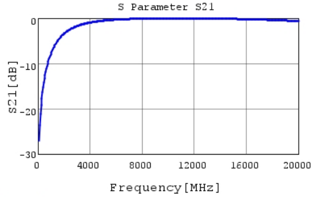
GJM0335C1ER70BB01 S21 DCOV, 25degC
