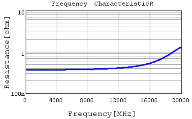
GJM0335C1ER70BB01 R DC0V, 25degC
