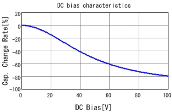
■ GCJ188R72A104MA01 C-DC bias capchange, 25.0degC, AC1.
