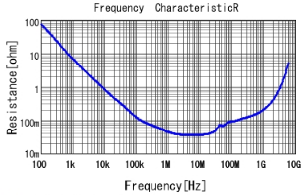
■ GCJ188R72A104MA01 R DCOV, 25degC
