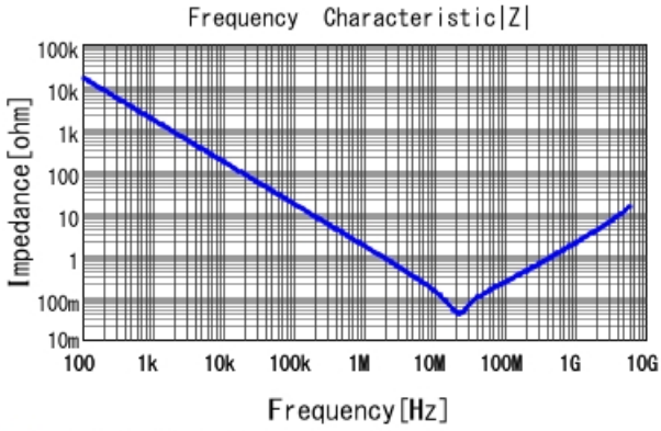
■ GCJ188R72A104MA01 |Z| DCOV, 25degC
