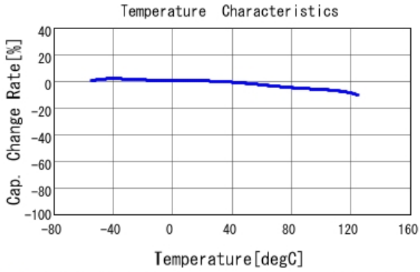
■ GCJ188R72A104MA01 C-Temp. capchange, DCO. 0V, AC1. 0Vrm
