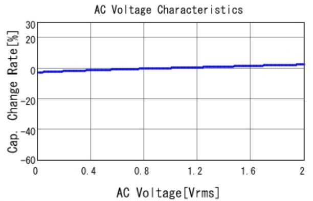
■ GCJ188R72A104MA01 C-AC Voltage capchange, DCOV, 25.0d
