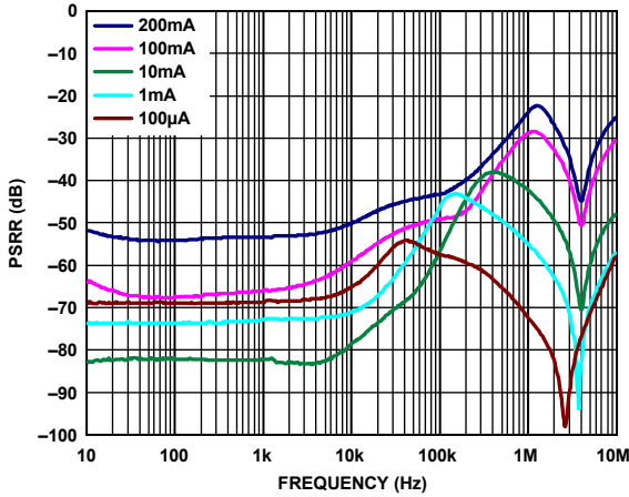
Figure 19. PSRR vs. Frequency, V_{OUT} = 3.3V , V_{IN} = 3.8V
