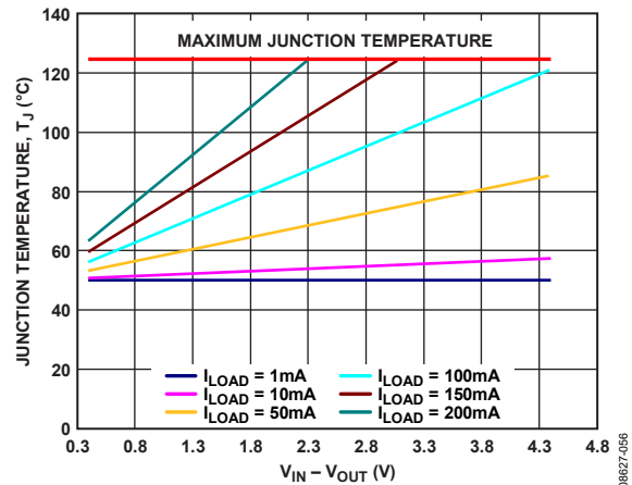
Figure 55. LFCSP 100 mm 2 of PCB Copper, T_A = 50^\circ\text{C}
