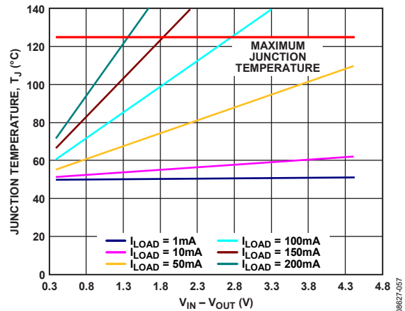
Figure 56. LFCSP 50 mm 2 of PCB Copper, T_A = 50^\circ\text{C}
