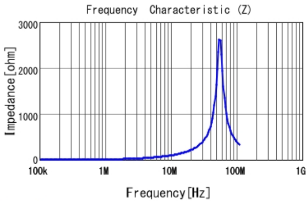
DFE252008U-1R5M |Z|
