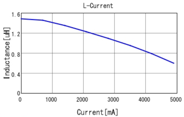
DFE252008U-1R5M L-Current 20degC
