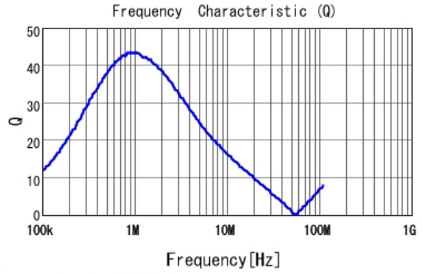
DFE252008U-1R5M Q
