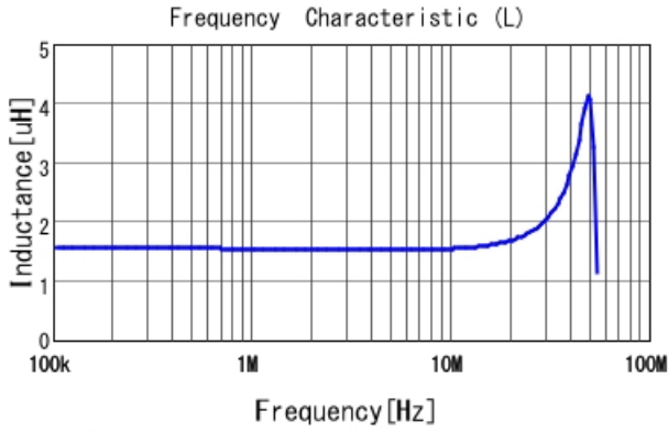
DFE252008U-1R5M L
